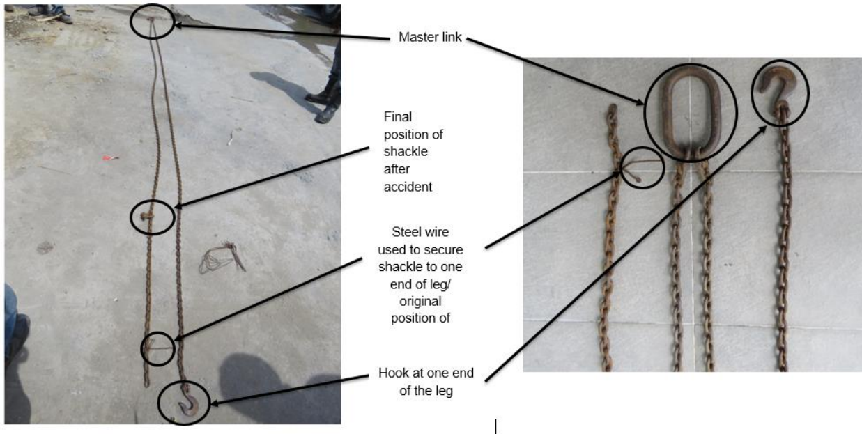
Images 4 and 5: Lifting Chain After the Accident
