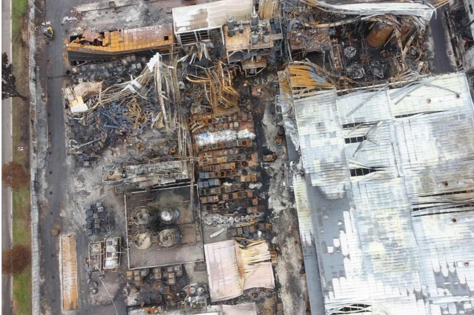
Photo 1: Aerial view of the incident scene at 23 Tuas View Circuit
