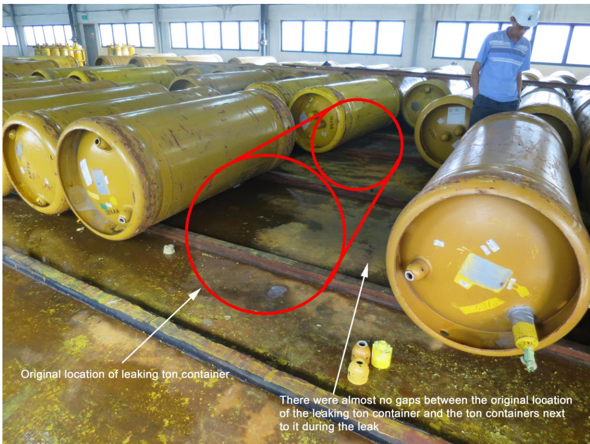
Photograph showing the original location of the leaking ton container (container has been removed in the above photo)
